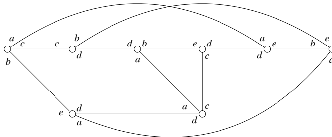
Figure 2: A 3-regular undirected graph requiring 5 colours.
