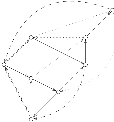
Figure 1: A 2-regular directed graph requiring 4 colours.
