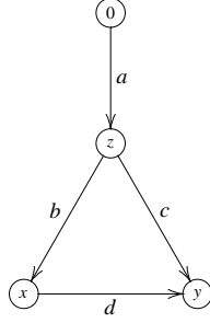
Figure 3: Property A_3 in action.
